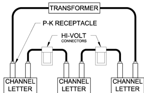
TYPICAL SIGN LETTER INSTALLATION
