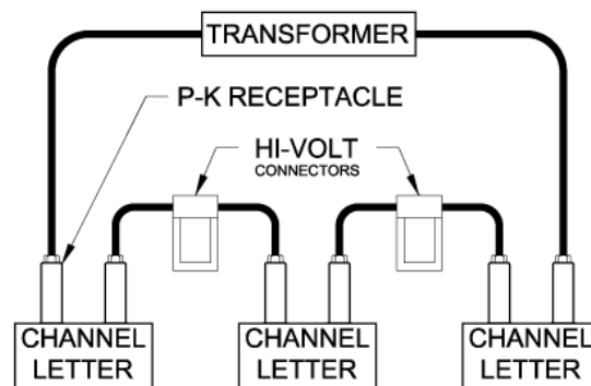
TYPICAL SIGN LETTER INSTALLATION
